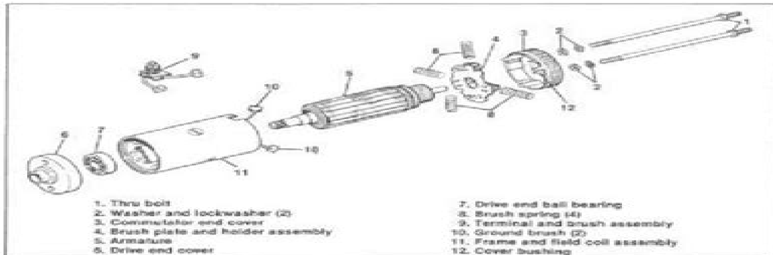
Figure 5-2. Starter Motor
