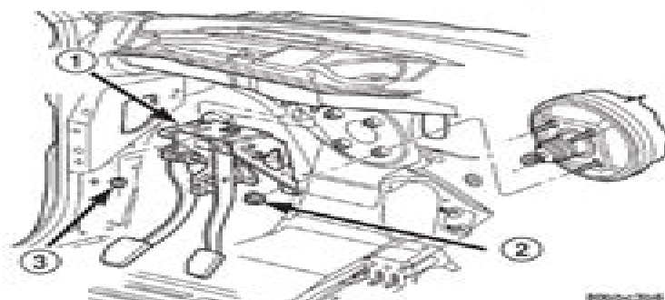
Fig. 40 Brake Pedal Mounting
