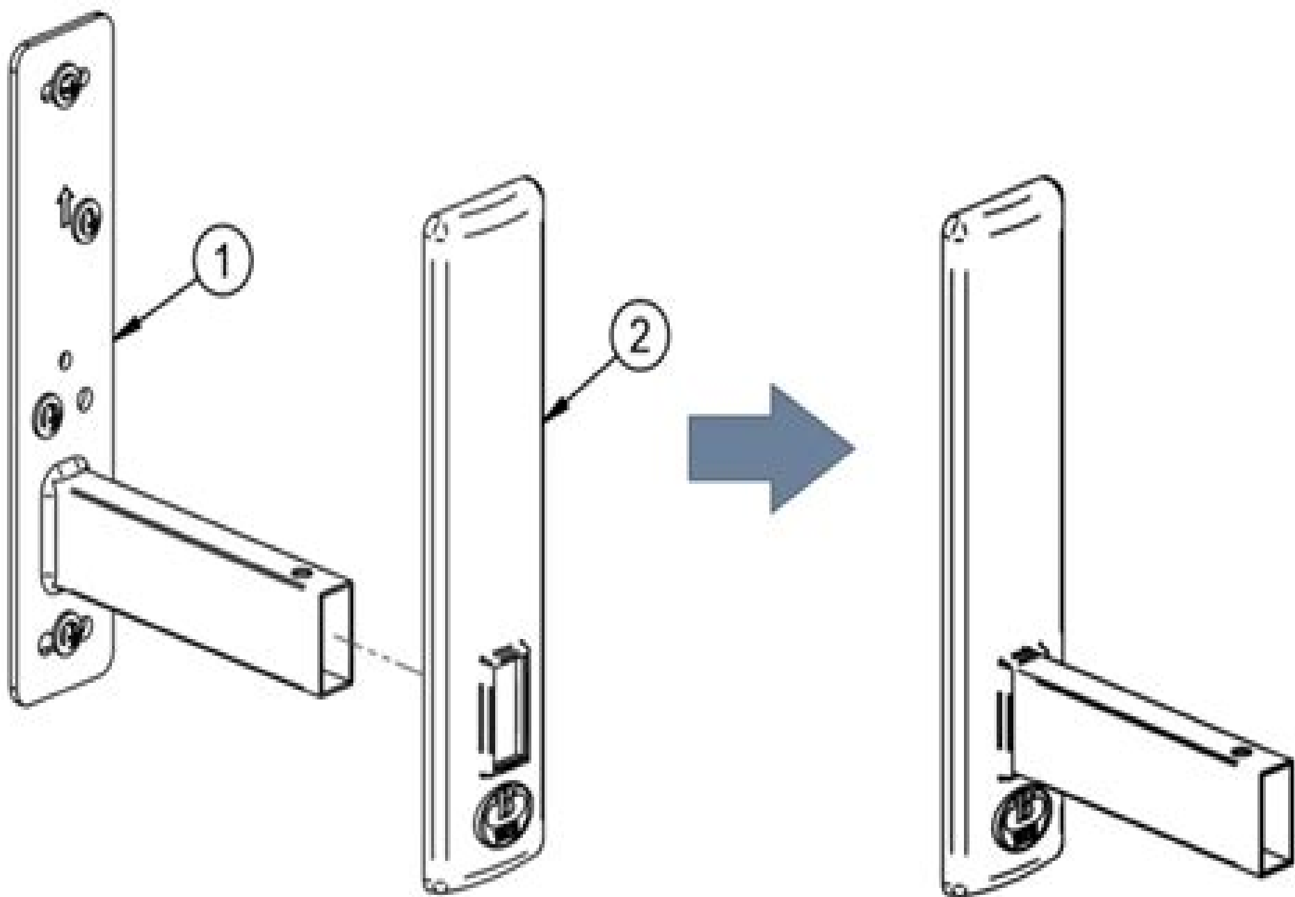
Figure 4: Sliding the Cover over the Wall Bracket
