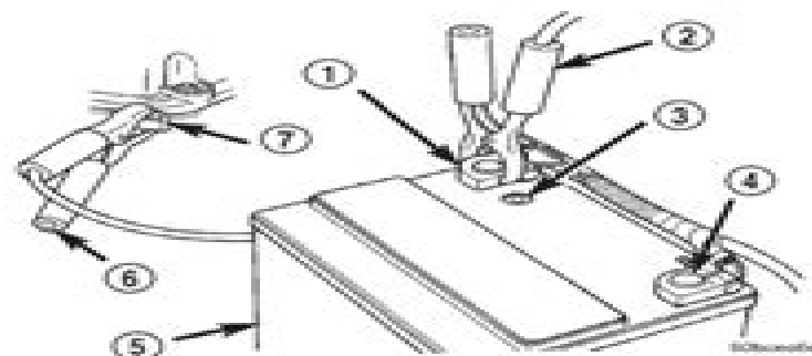
Fig. 1 Jumper Cable Clamp Connections
