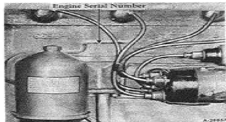
Illustr. 2A Location of engine serial number.
